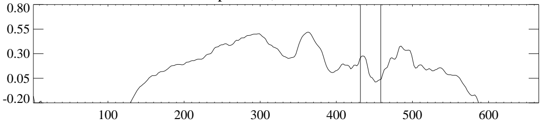
upshifted, alt > 529 km
