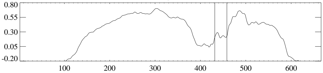
downshifted, alt > 529 km
